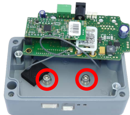
Image 10: DIN rail screws
